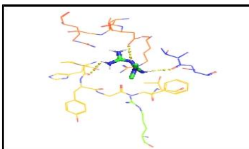
Ligand binding
