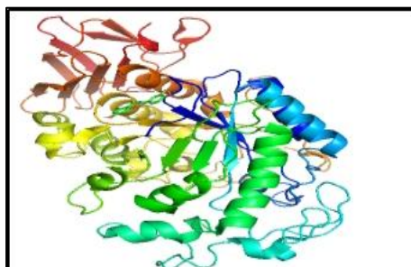
4W93 luteolin
