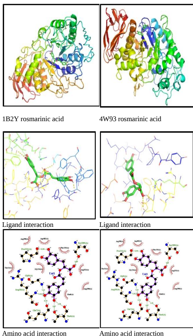
Figure 8: Docking of ligand rosmarinic acid with 1B2Y and 4W93 and their interactions shown in two columns respectively.
