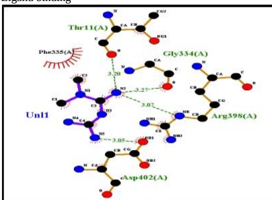
Ligand binding
