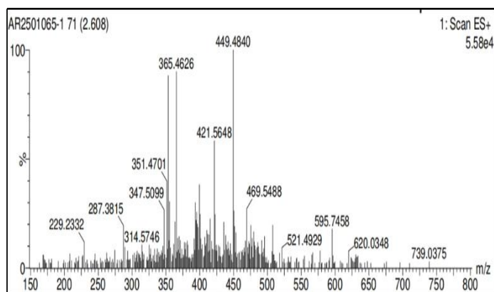
Figure 3 b: LC-MS Profiling of Petroleum ether extract of Mentha arvensis leaves.
