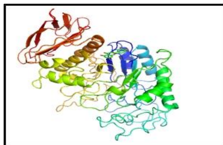
1B2Y luteolin
