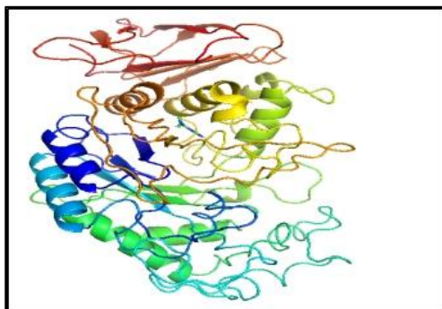
1B2Y metformin
