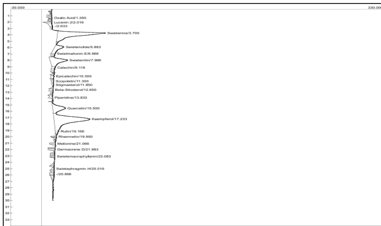
Figure 1: HPLC Chromatogram of Swietenia mahagoni Extract Showing Peaks Corresponding to Phytochemicals Listed in (Table 1)
