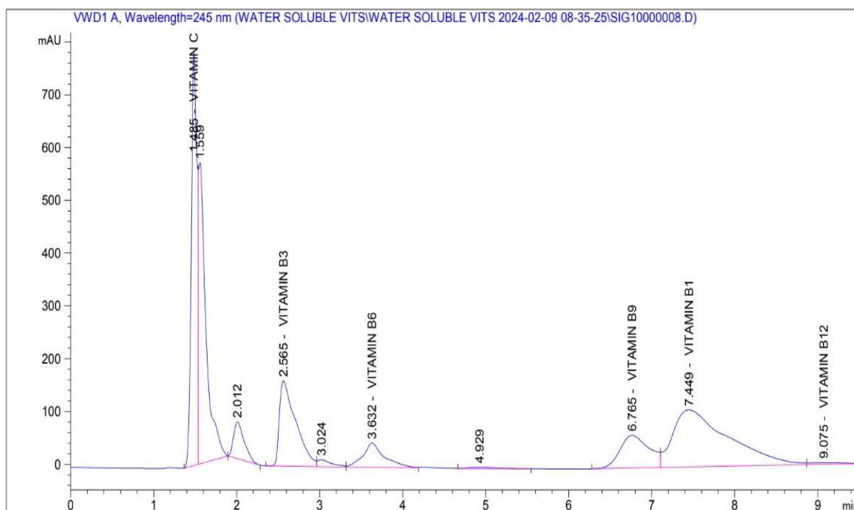
Figure 3: HPLC chromatogram of standard mixture of water-soluble vitamins showing retention times
